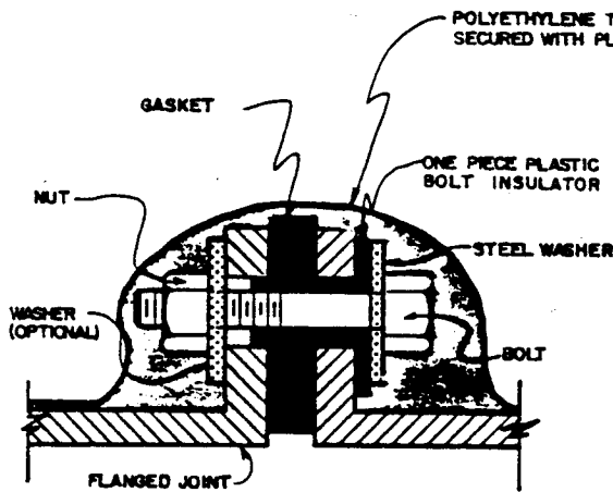
INSULATED FLANGE JOINT
