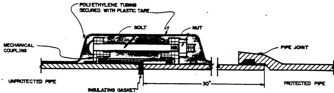
INSULATED MECHANICAL COUPLING
