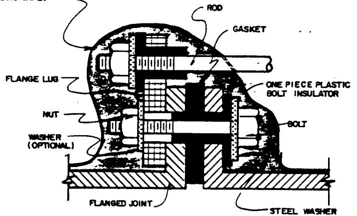
INSULATED TIE BACK ROD
