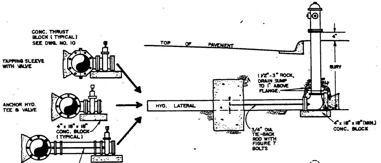
PROFILE showing 3 acceptable valve and tee fittings.
