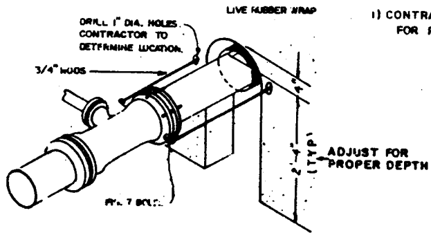
DETAIL 'A'-Pipe Arch
